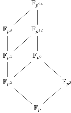
FIGURE 5.1. The subfields of \mathbb{F}_{p^{24}}
